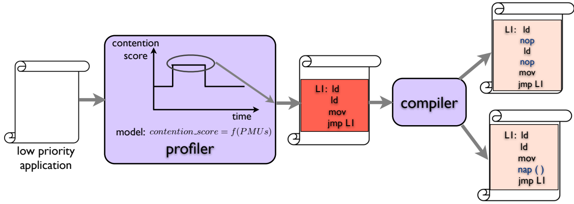
Figure 2: QoS-Compile Overview
