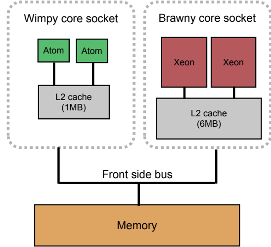
Fig. 12: Heterogeneous processor platform (Intel’s QuickIA)
