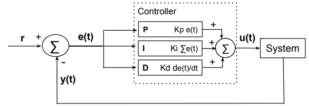
Fig. 7: Basic elements of the PID control system
