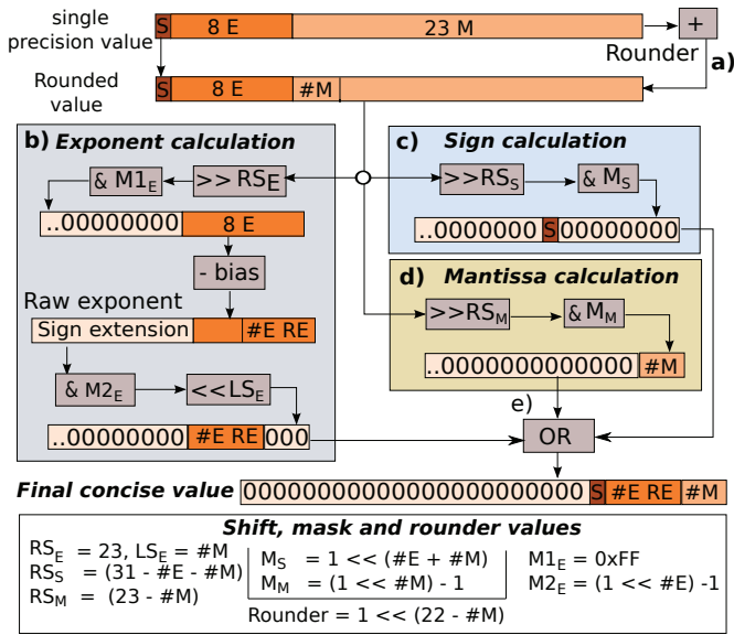
Fig. 8. Block diagram of Exact to Concise unit
