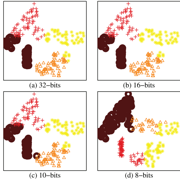
Fig. 1. Kmeans clustering output when applying a range of different storage formats. Similar accuracy for 32 (precise), 16 and 10 bits but poor accuracy for 8 bits
