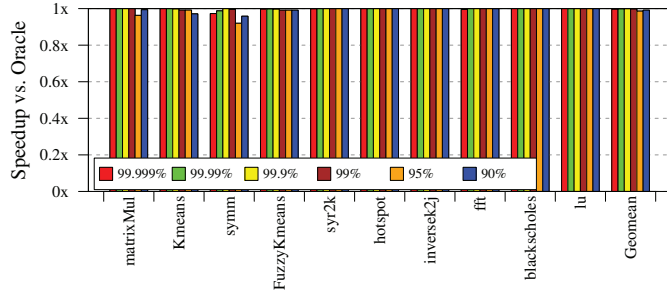
Fig. 13. Comparison of FSA-chosen configuration performance against an oracle format selector. The FSA achieves > 98% of oracle performance on average
